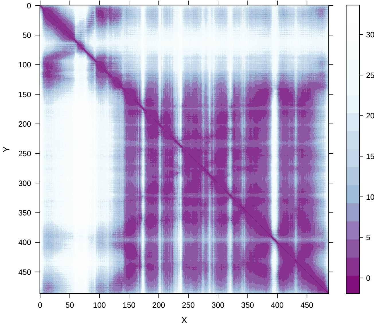
PAE | Bunzi.Bunzi__BnzB.0.V-plddts_86.65253
