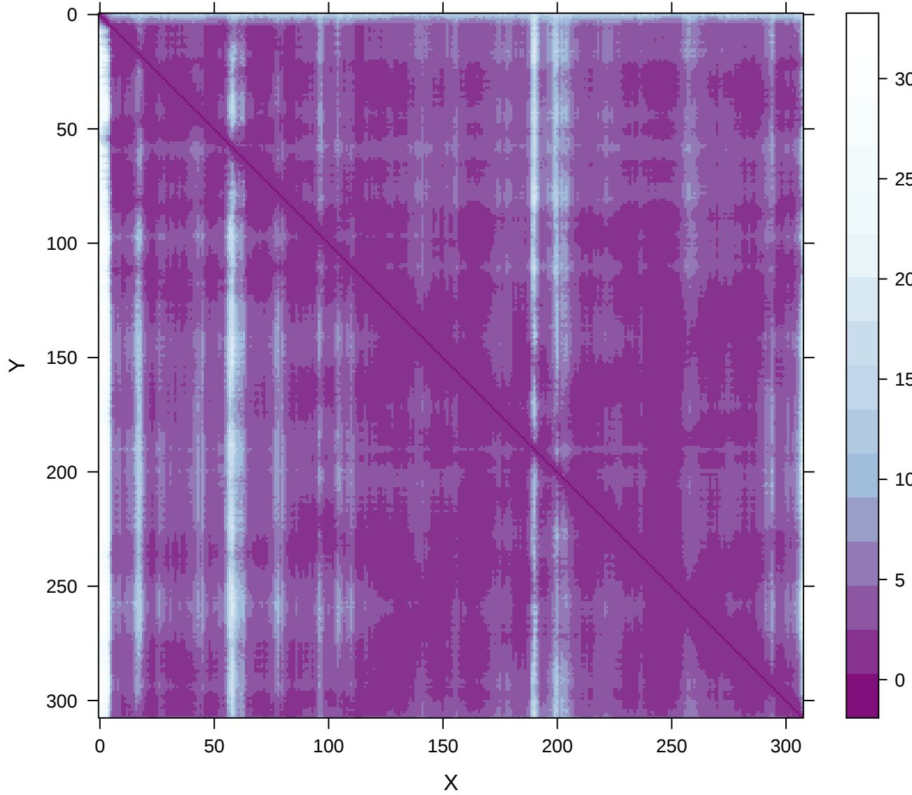
PAE | PARIS_II.Rst_PARIS__DUF4435.0.V-plddts_95.47009
