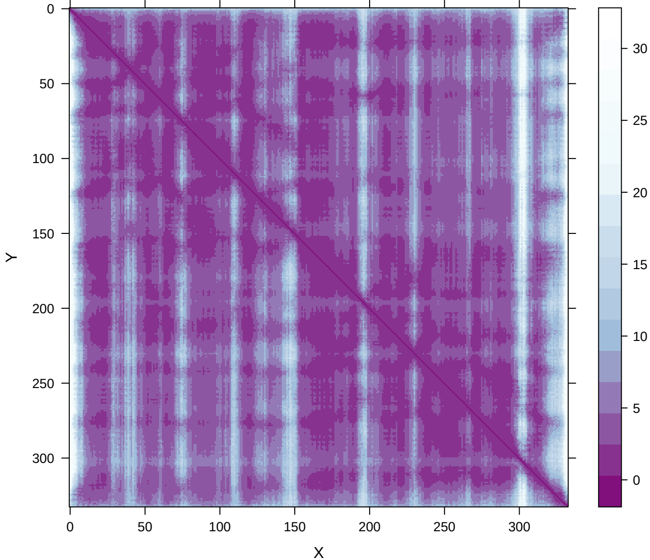
PAE | Rst_3HP.Rst_3HP__Hp1.0.V-plddts_92.14077
