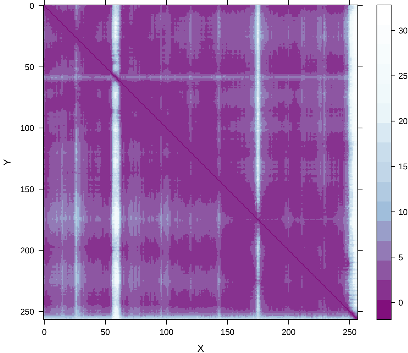
PAE | Septu.Septu__PtuB.0.V-plddts_95.60363
