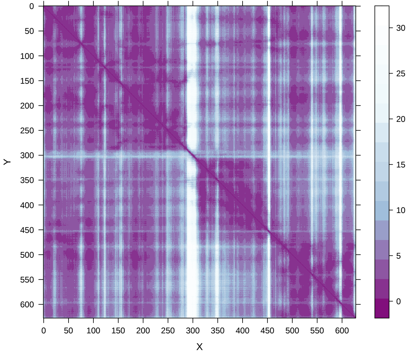
PAE | AbiA_large__AbiA_large-plddts_90.82916
