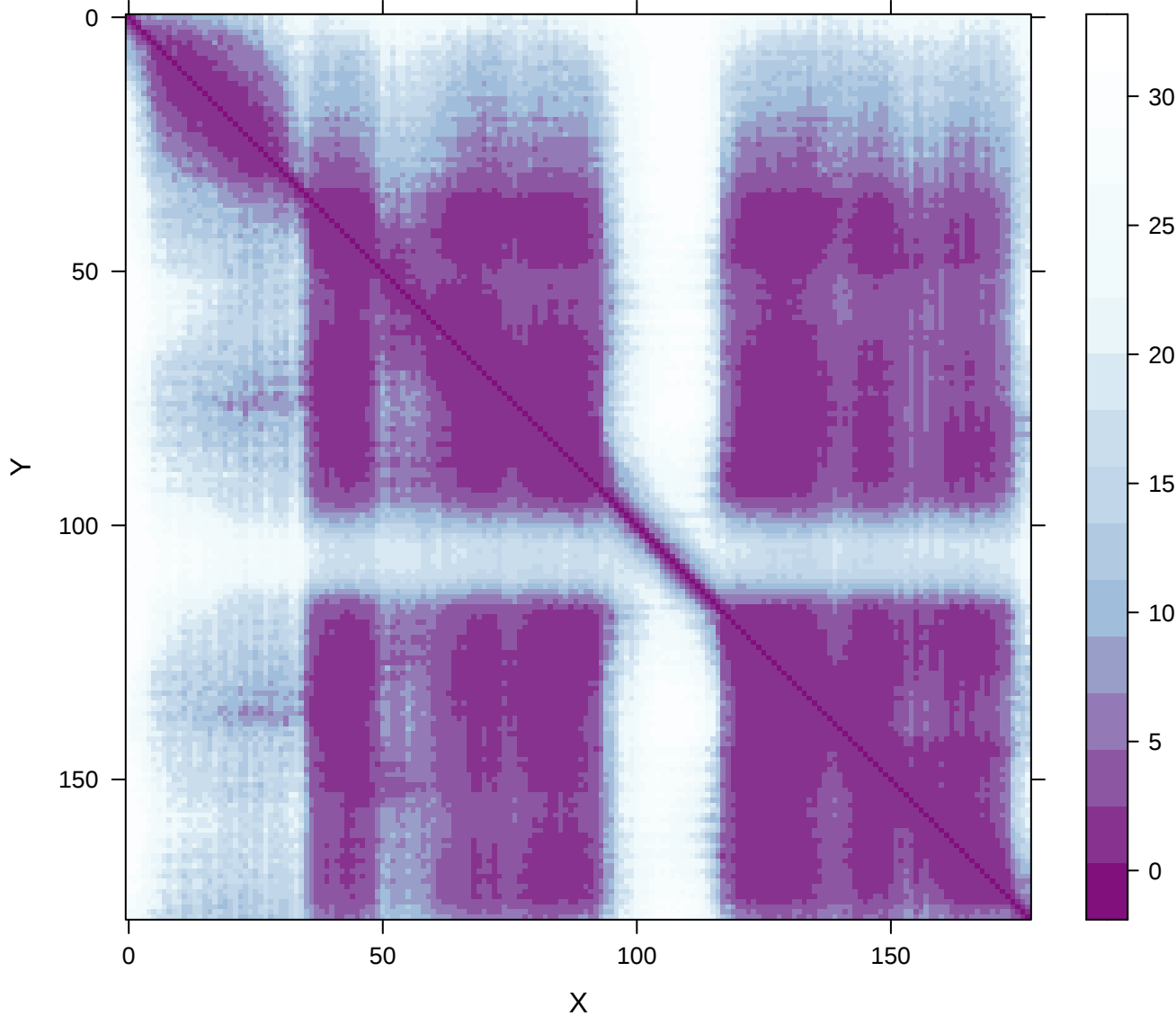
PAE | AbiN__AbiN-plddts_84.27216
