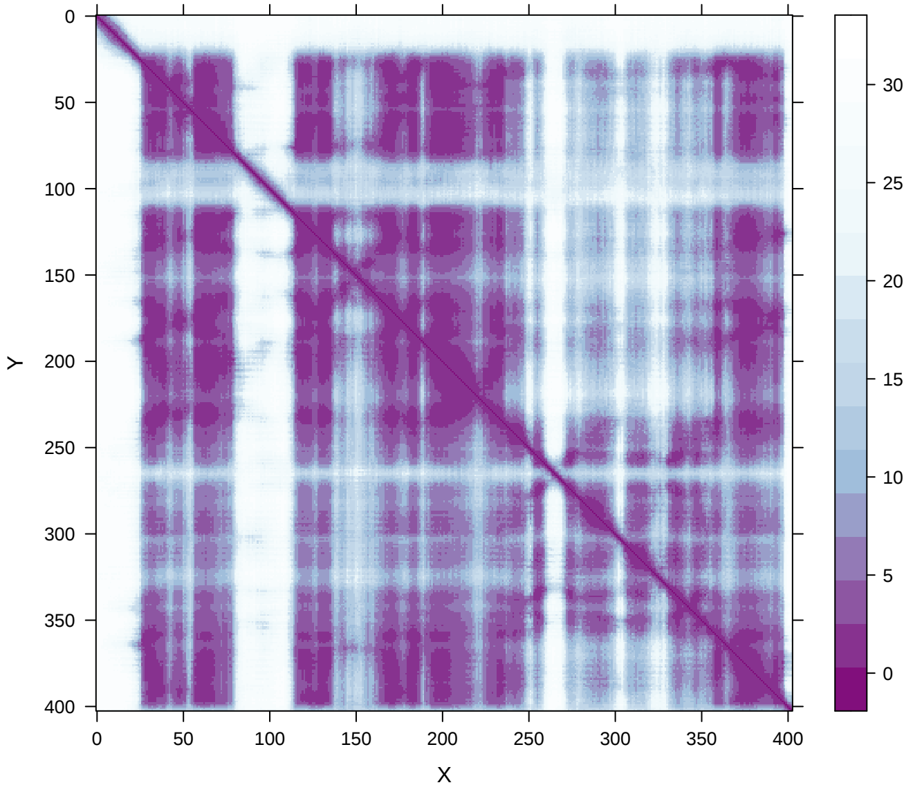
PAE | Butters_gp30_gp31__Butters_gp30-plddts_79.33298
