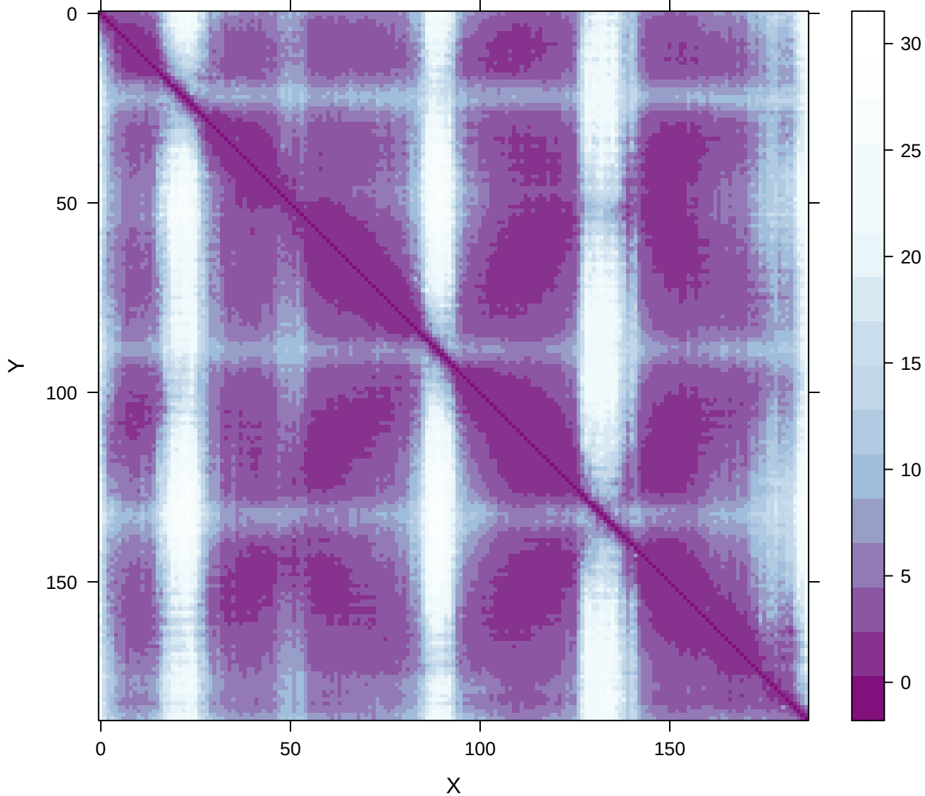
PAE | Butters_gp30_gp31__Butters_gp31-plddts_84.75463
