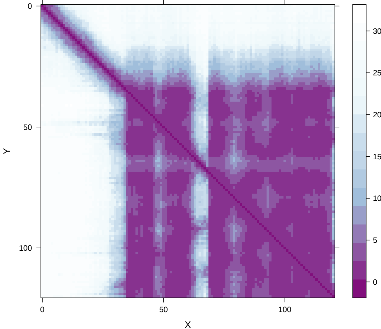
PAE | Charlie_gp32_gp32-plddts_82.99758
