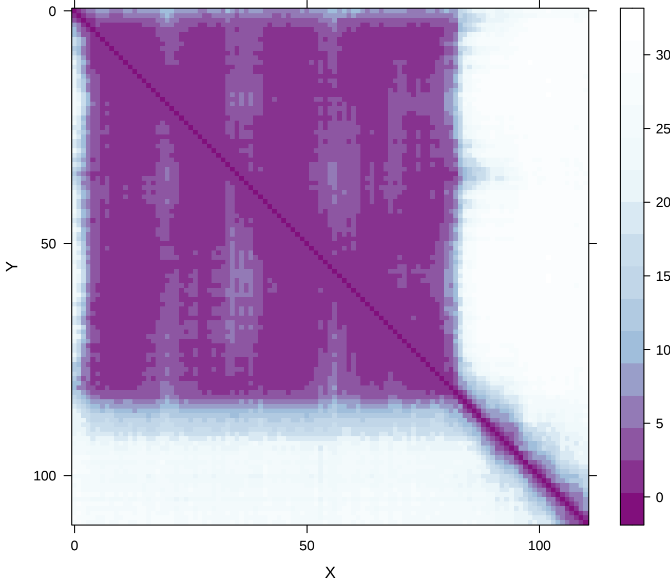
PAE | GAPS6__GAPS6a-plddts_82.29413
