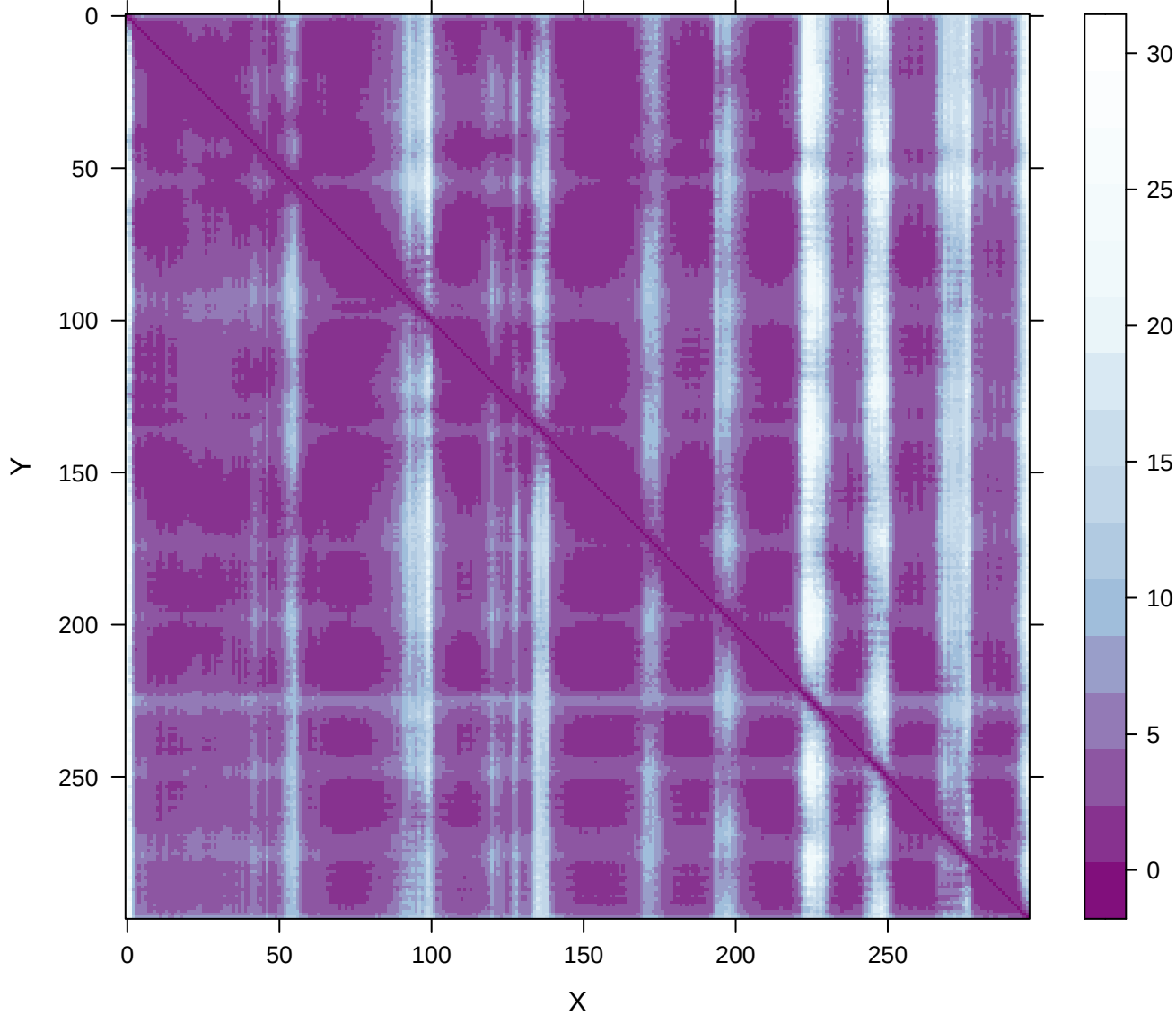
PAE | Lit_Lit-plddts_91.19971
