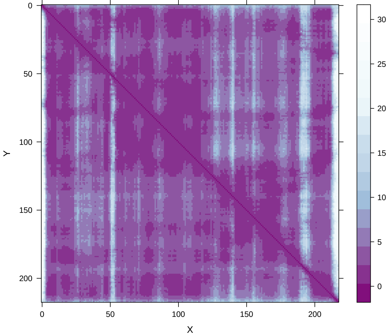
PAE | MADS__mad4-plddts_92.44061
