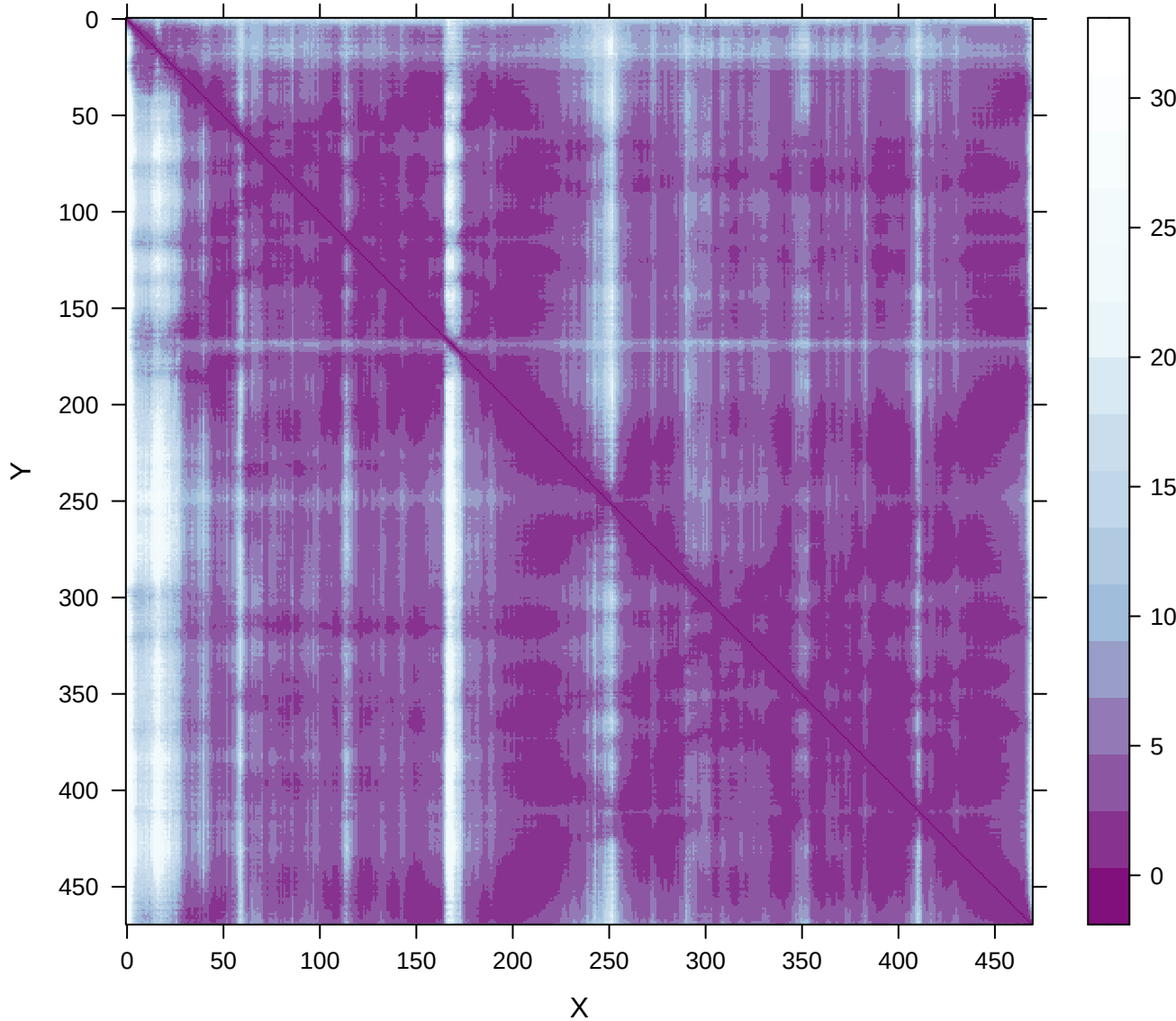
PAE | MADS__mad5-plddts_93.90587
