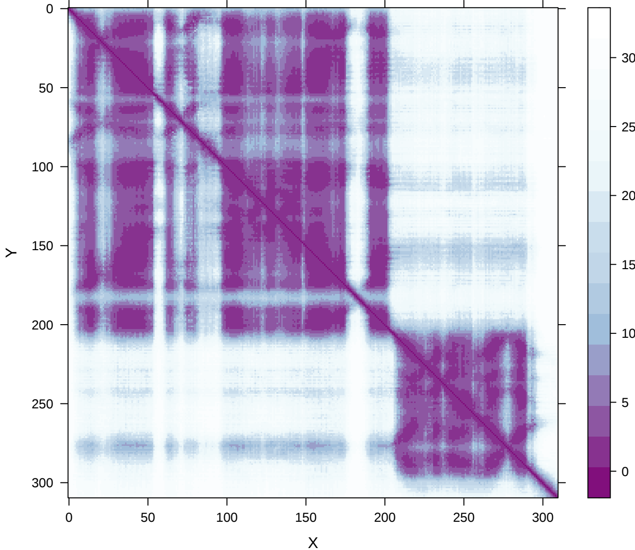
PAE | MMB_gp29_gp30_gp29-plddts_82.71079
