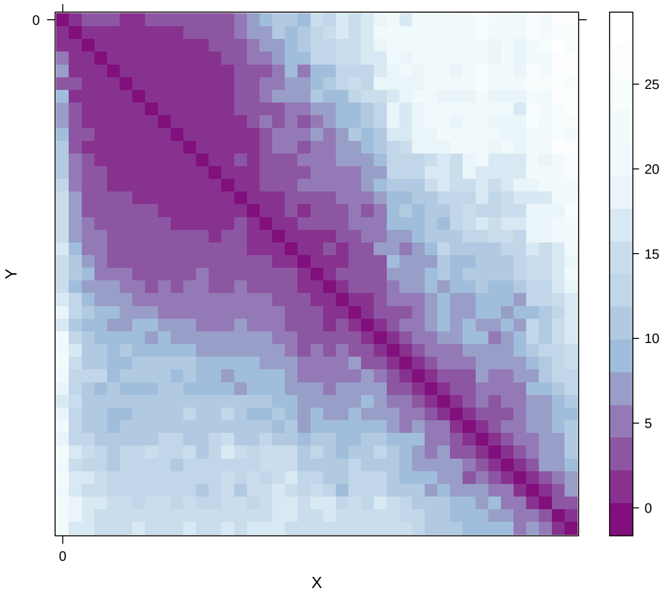
PAE | Mok_Hok_Sok__Hok-plddts_80.98652
