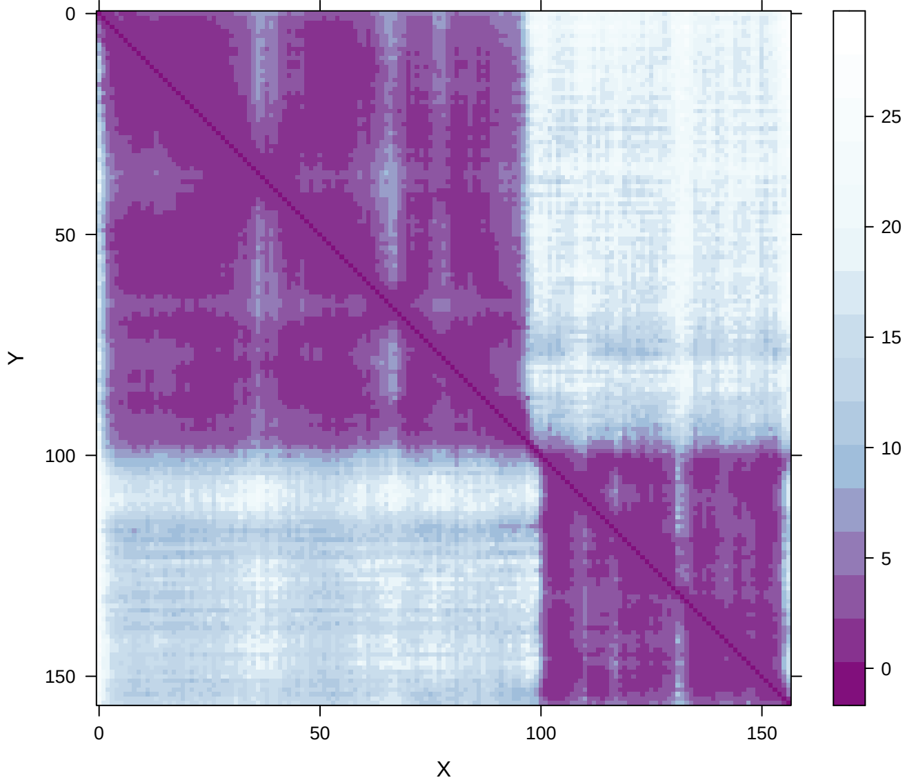
PAE | Nixl__Nixl-plddts_92.38782
