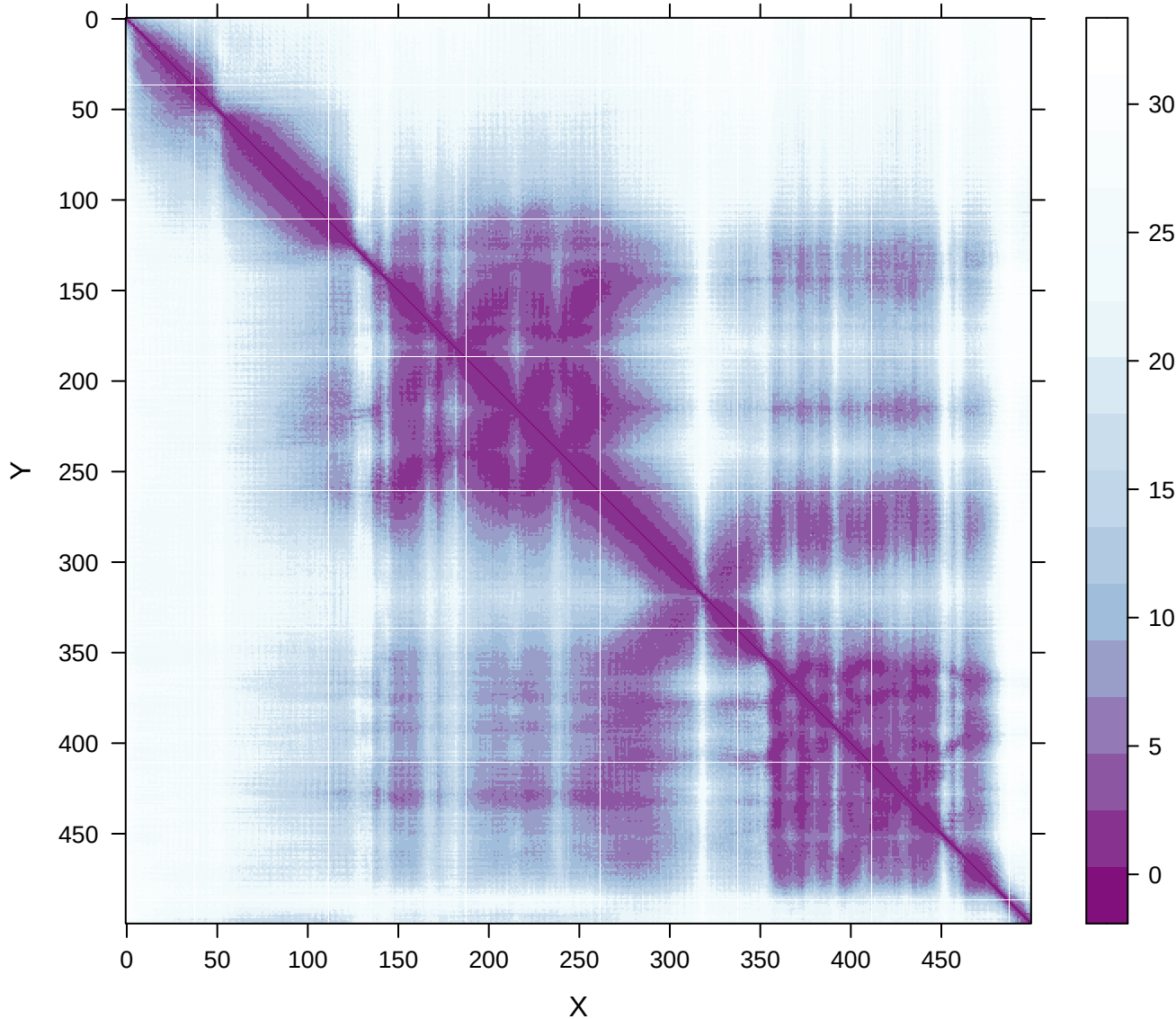
PAE | PD-Lambda-1__PD-Lambda-1-plddts_85.64965
