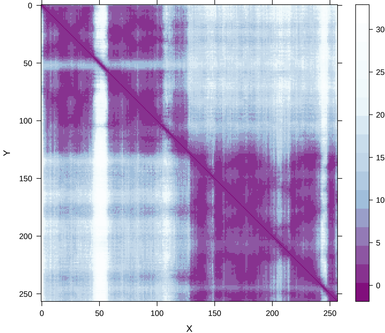
PAE | PD-T4-3__PD-T4-3-plddts_88.02514
