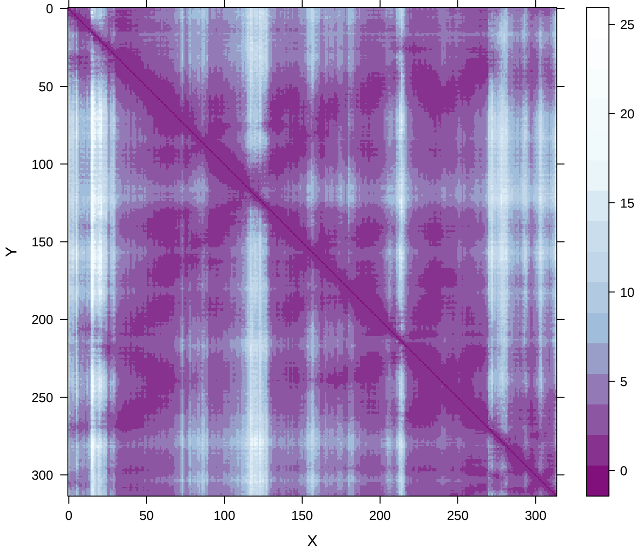
PAE | PD-T4-5__PD-T4-5-plddts_94.58803
