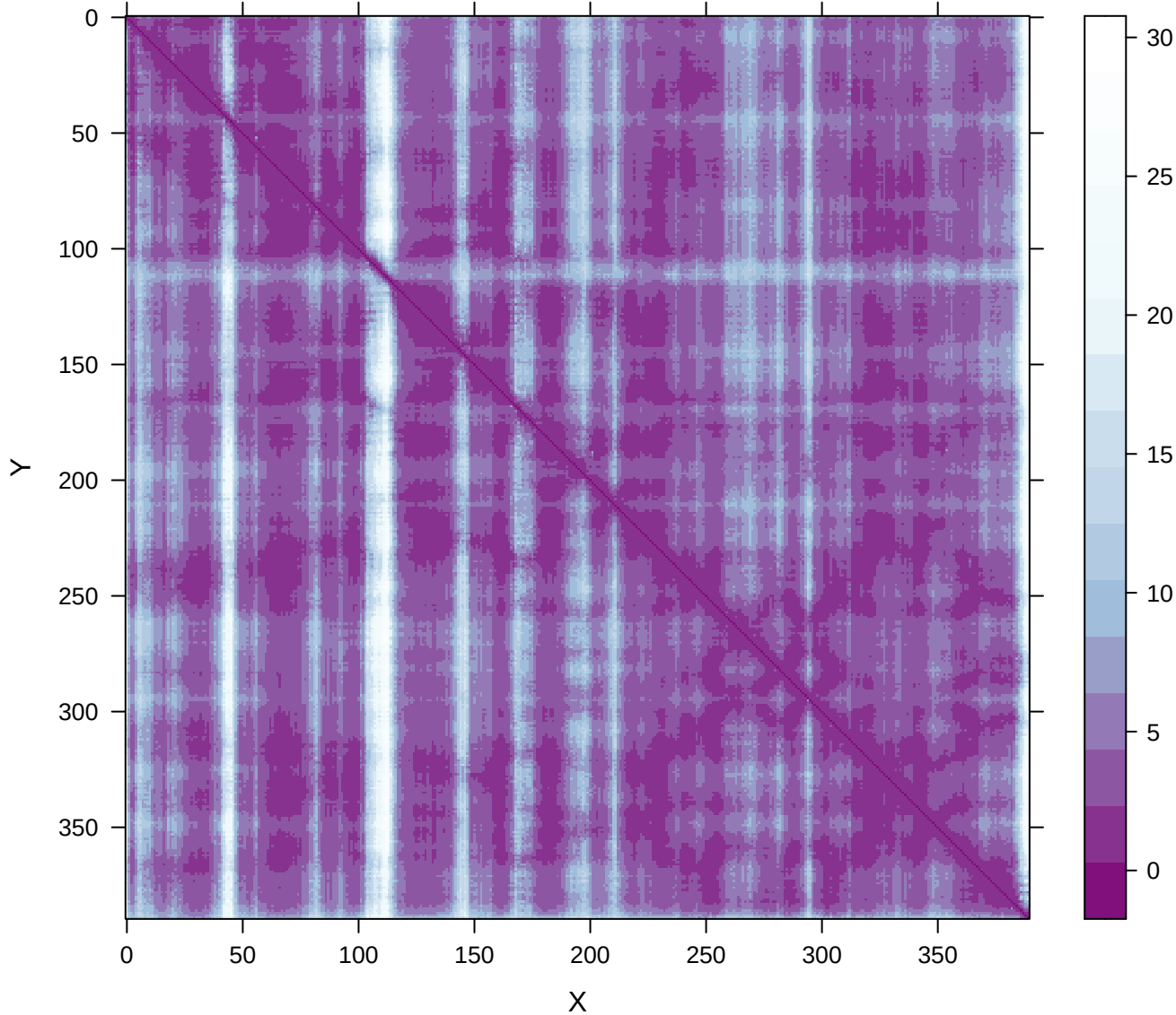
PAE | PD-T7-5__PD-T7-5-plddts_92.01228
