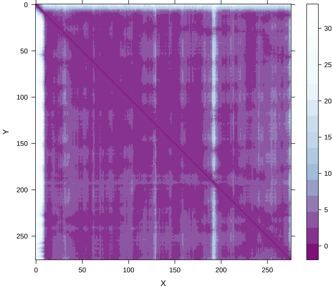
PAE | Viperin__pVip-plddts_95.08271
